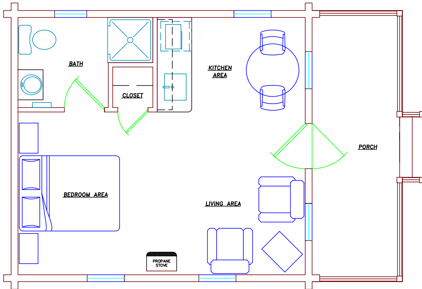
CABIN "A" FLOOR PLAN 20
