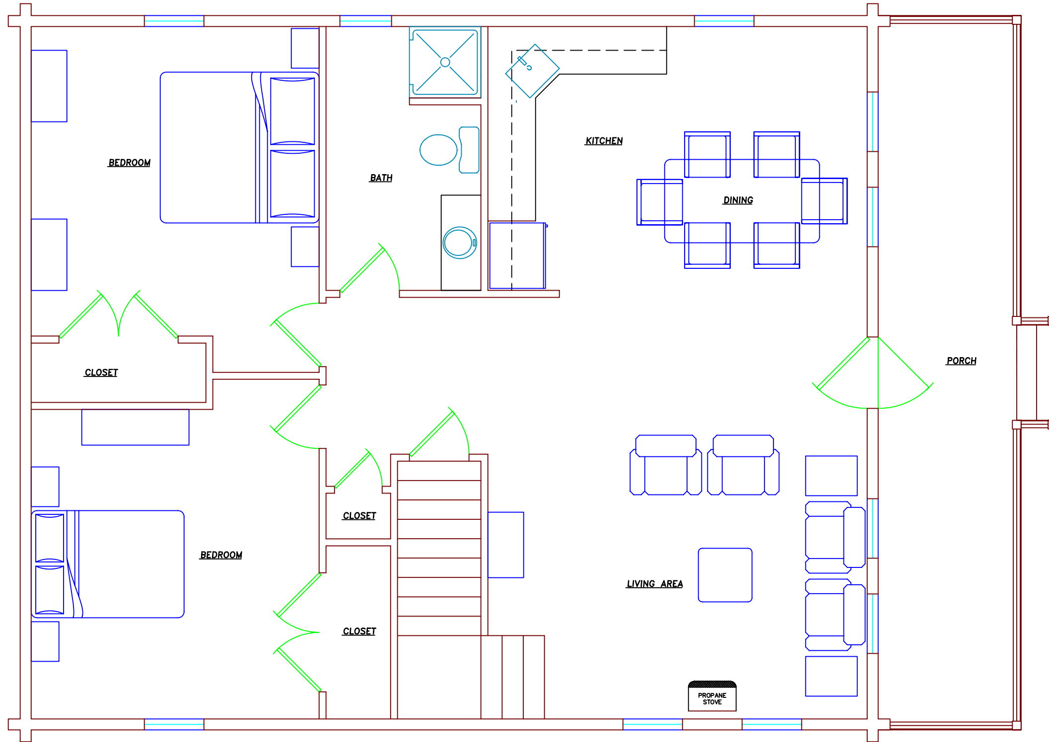
CABIN "F" FIRST FLOOR PLAN (10)
